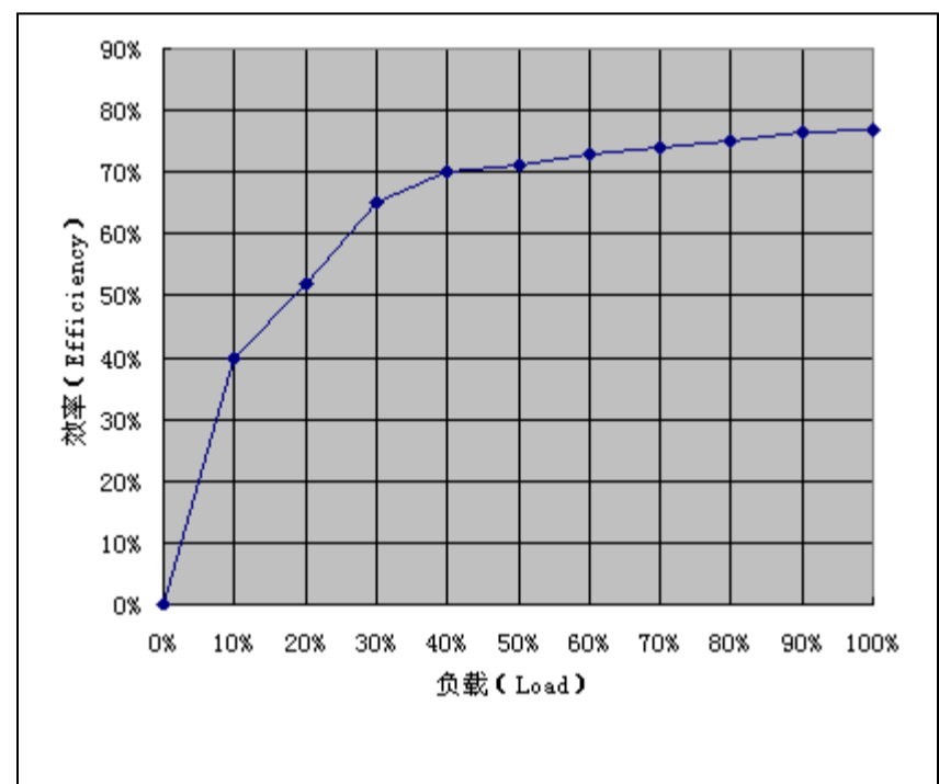
效率曲线 Efficiency curve
