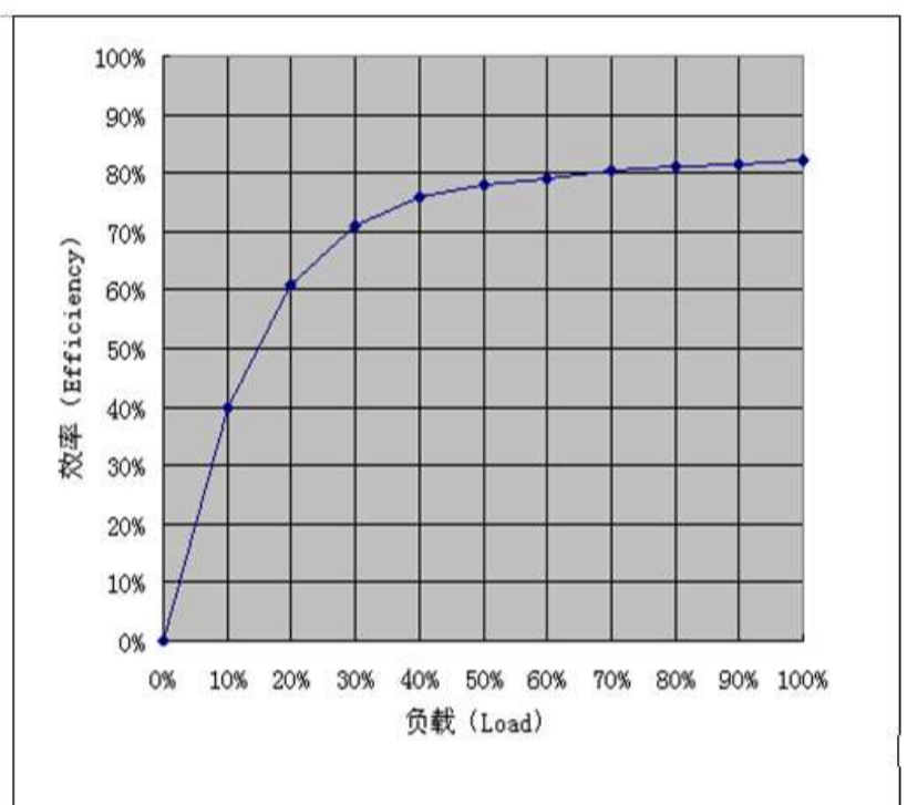
Efficiency curve
