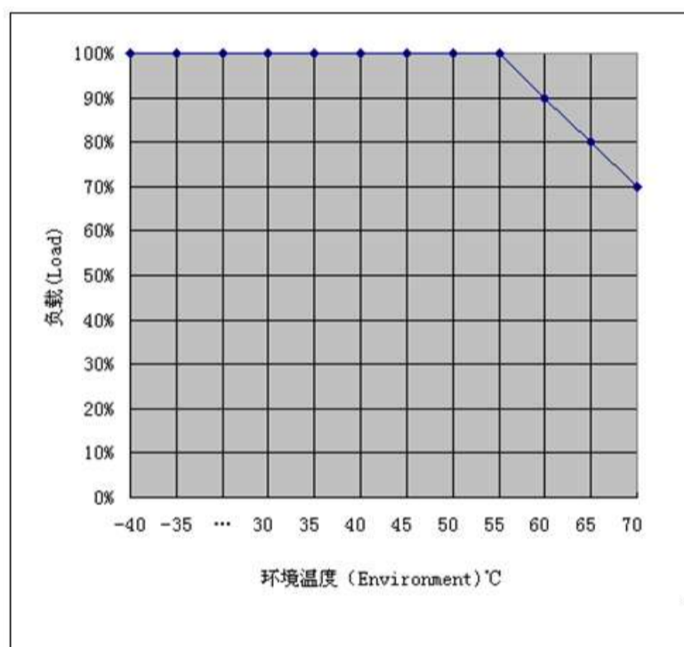
Derating curve
